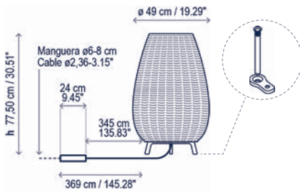
Wet Rated connection box with driver included / Caja de conexión estanca con driver incluido
